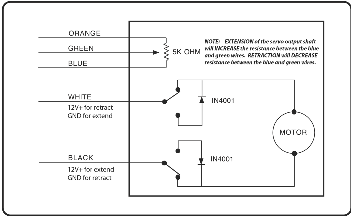
Figure 1 B6 actuator internal wiring diagram.
